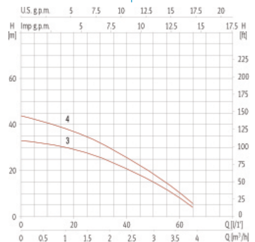
Performance curve at 2900 rpm
